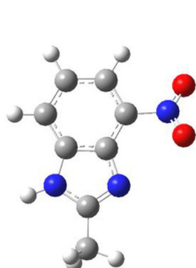
2-methylbenzimidazole
