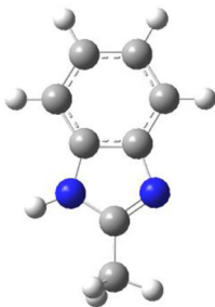
2-methylbenzimidazole
