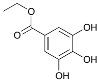
ethyl gallate, EG
