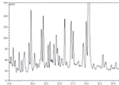
Phenols
