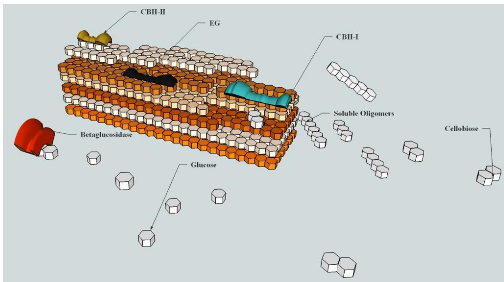
Figure A2.1 Action pattern of cellulase enzymes simulated in the model
