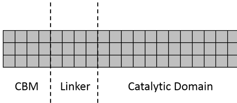
Figure A2.2 Shape of cellulase used in the model. Each block represents a glucose molecule (modified from Levine et al.)
