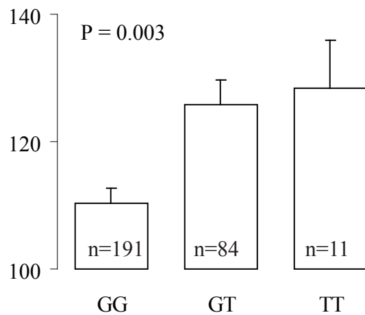
2677 G>T genotypes
