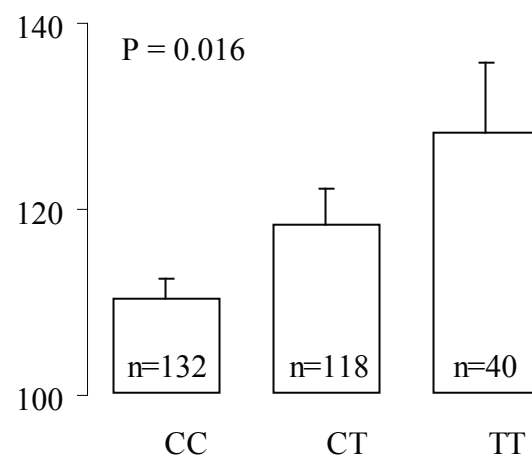
3435 C>T genotypes
