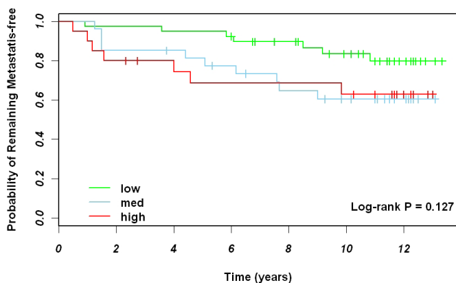
E. Wang et al., unadjusted ROR-S
