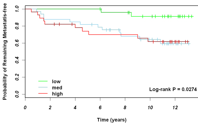
F. Wang et al., 10% normal-adjusted ROR-S
