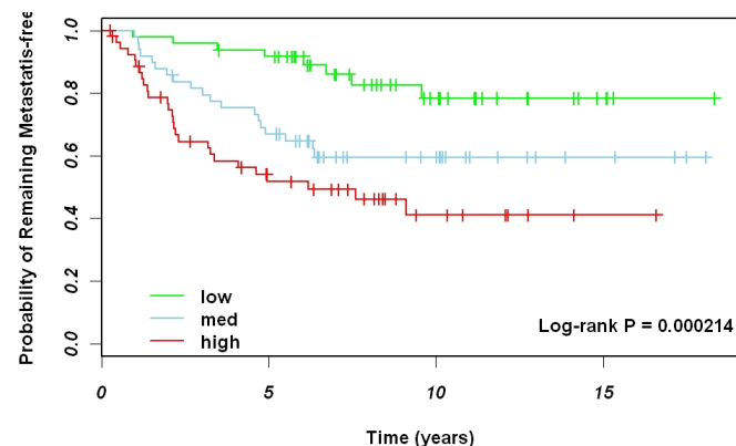
D. Naderi et al., 20% normal-adjusted ROR-S
