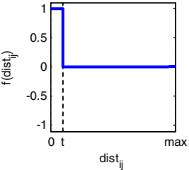
ReliefF
