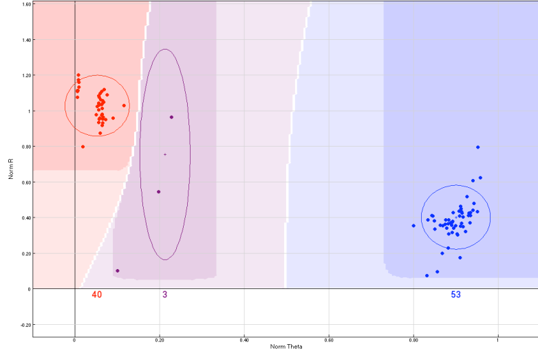
C. rs10096900
