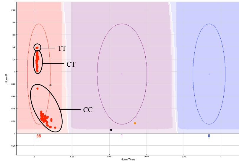
A. rs10786712
