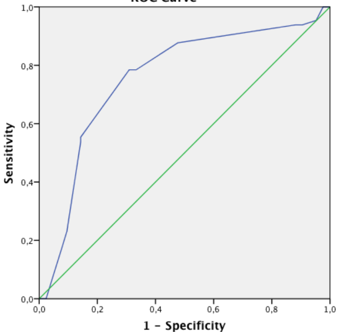
ROC Curve
