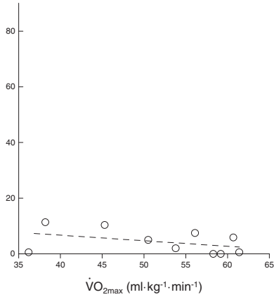
(c) CAT
