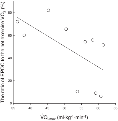
(a) SIT
