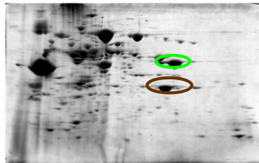
C (SF370 \Delta covS )
