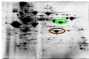
D (1529 \Delta covS )
