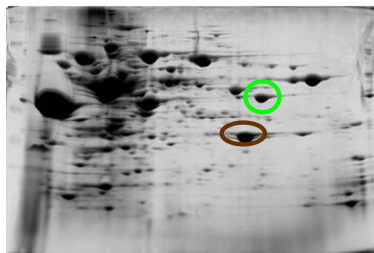
B (GT01 \Delta covS )
