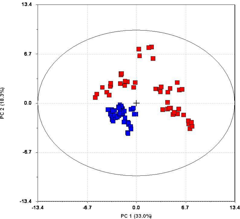
PCA Score Plot of all mean peak intensities in m/z are a 2 kDa - 25 kDa
