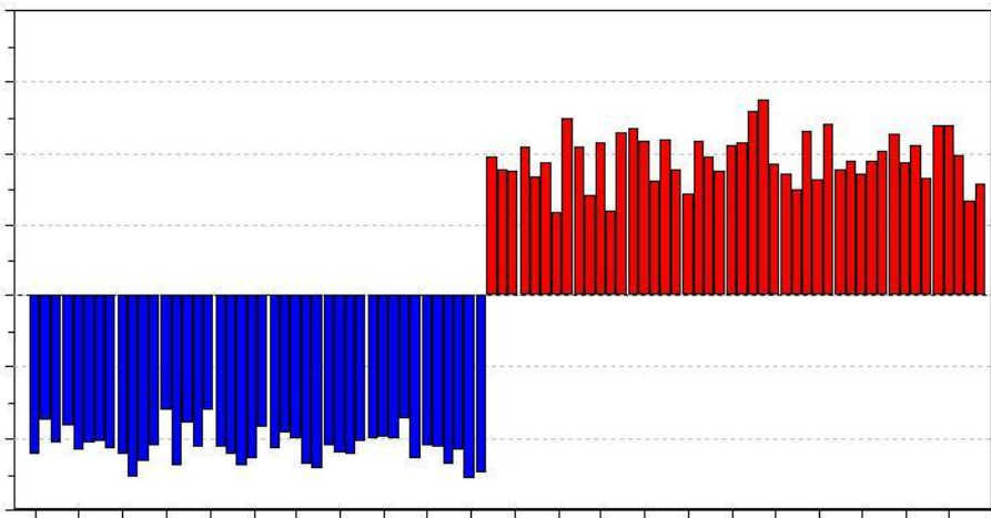
Target Projection Scores - 5 components
