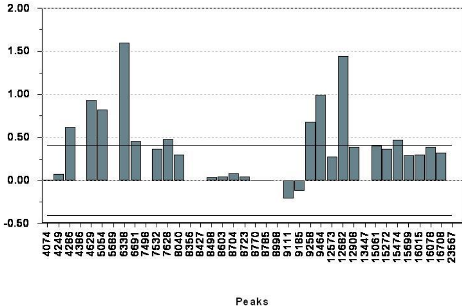
Selectivity Ratio Plot - All peaks
