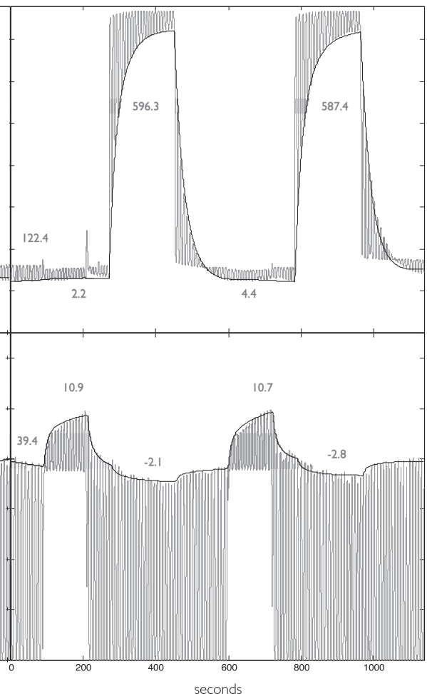
New breathing circuit – Run 2
