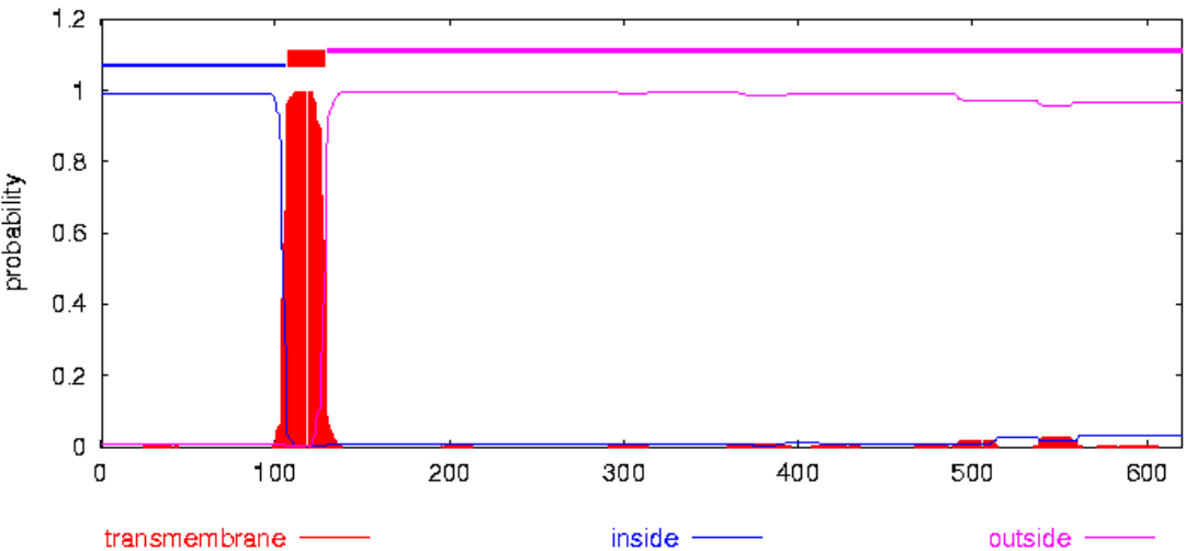
TMHMM posterior probabilities for Sequence
