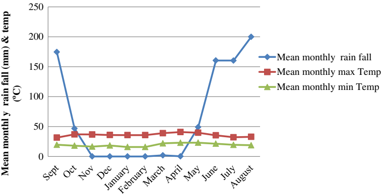
Mean monthly rain fall, maximum and minimum temperature from Baeker and Humera during 2011-2013
