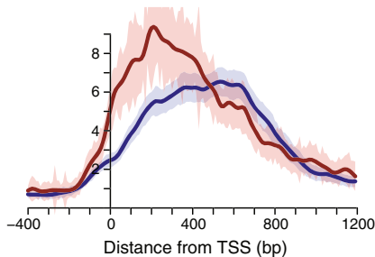
Intron-containing genes
