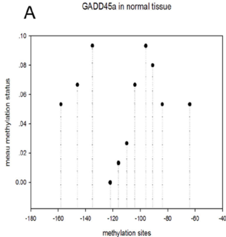
GADD45a in normal tissue
