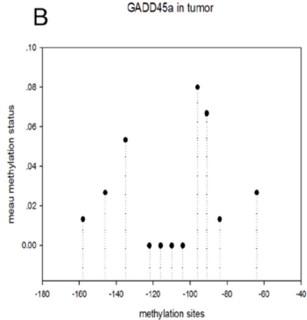
GADD45a in tumor
