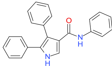
Molecular Framework 1
