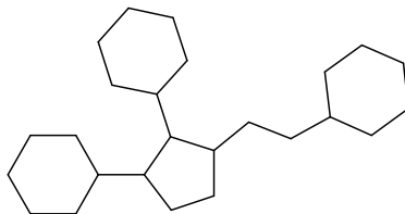
Graph Scaffold
