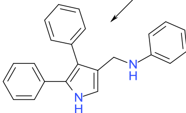
Molecular Framework 2
