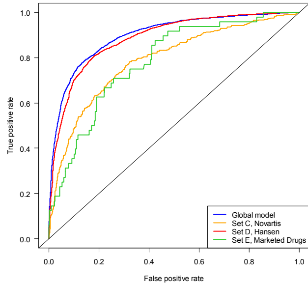
Performance in the global model, random forest OOB
