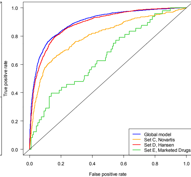
Local models, random forest OOB
