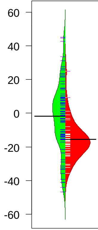
Nitrenium Formation Energy (relative kcal/mol)
