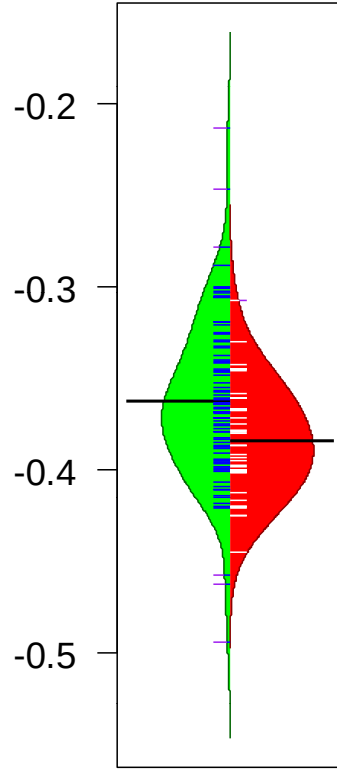
Nitrenium Natural Charge (e)
