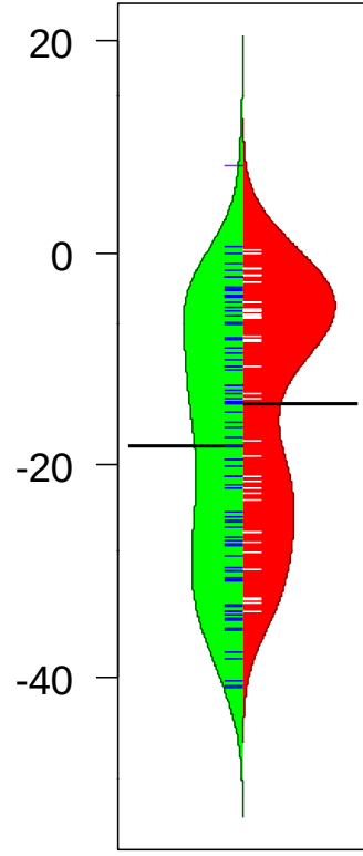
Anion Formation Energy (relative kcal/mol)
