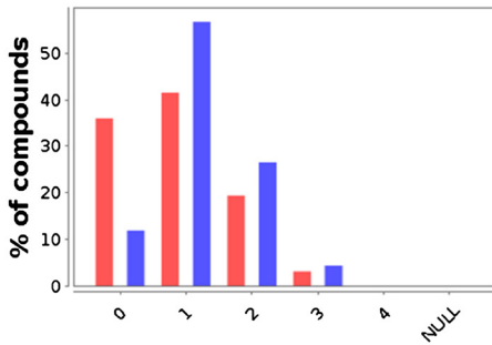
HBD
