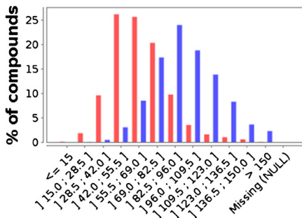
TPSA
