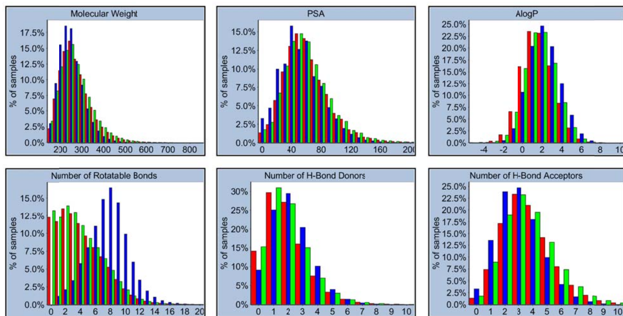
Supplemental Figure 1. Histogram analysis of enumerated structures with an olefin fragment included (see Experimental Section, Table 1 of the manuscript for details).
