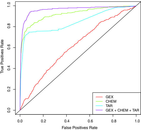
Kernels predictive power
