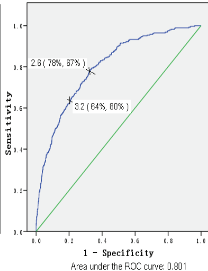
ROC curve analyses in pubertal subjects
