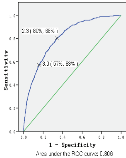
ROC curve analyses in total participants
