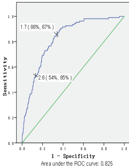
ROC curve analyses in prepubertal subjects
