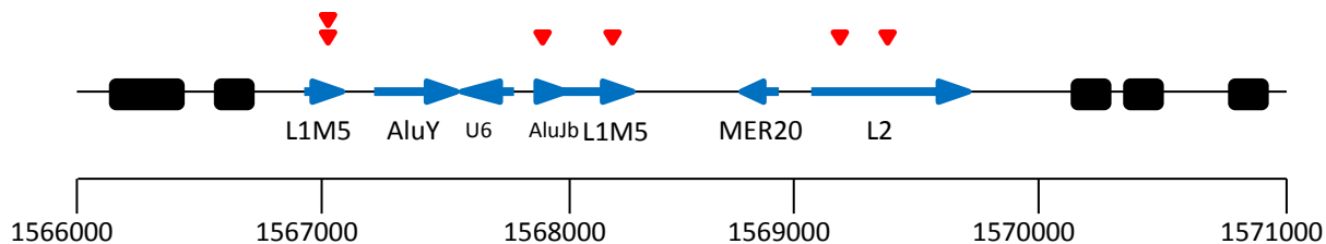
Genome coordinates for TCF3 translocation junction region (Chr19)
