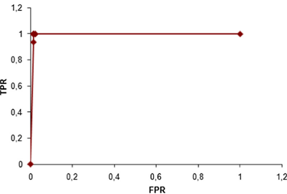
(c) ROCLLJ48W3xW2
