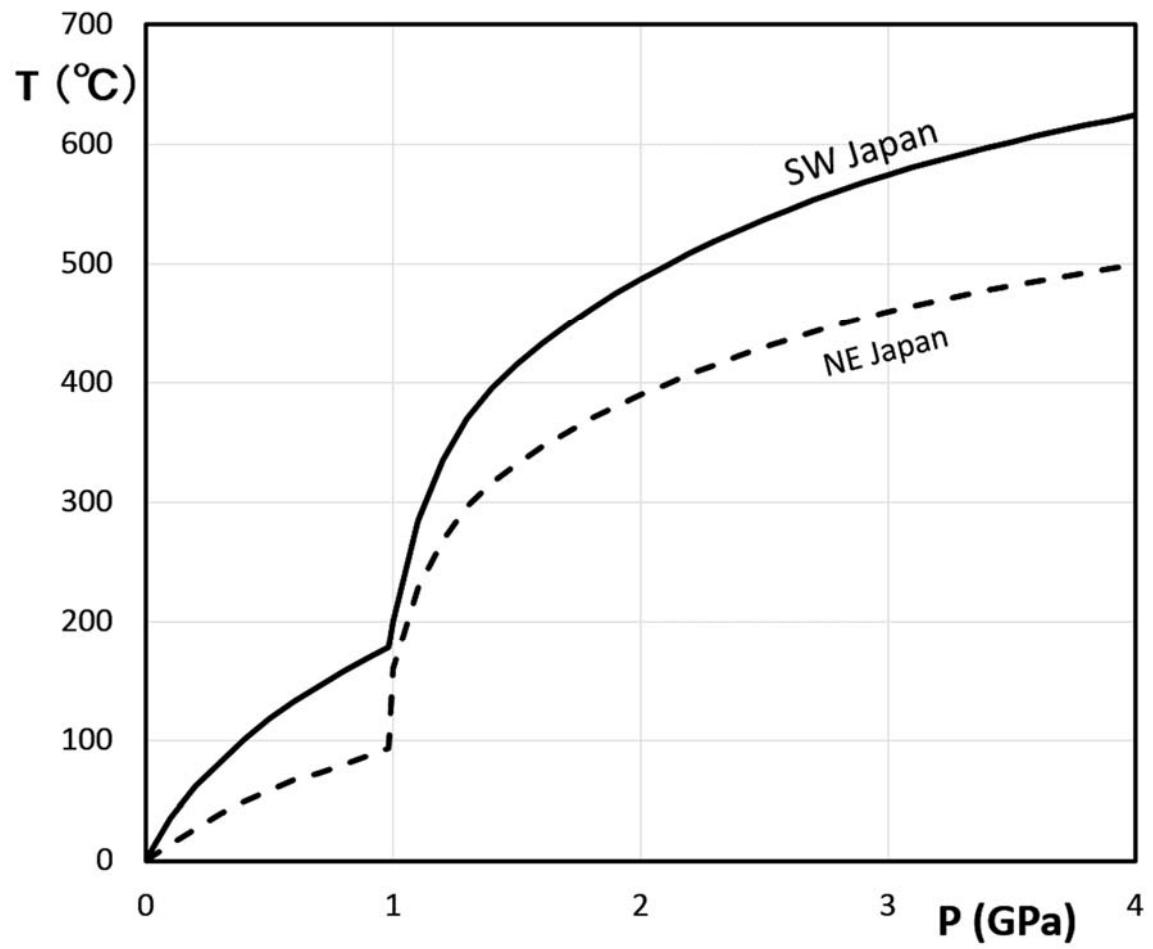
Fig.S1 Calculated geotherms along the subducting slab for southwest Japan (SW Japan) and northeast Japan (SE Japan), based on the formulation of England and Wilkins (2004), with the parameters listed in the main text.
