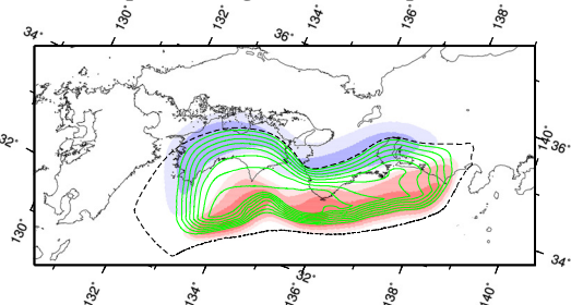
(c) Sub-slip 3 (Seismogenic + Down-dip)
