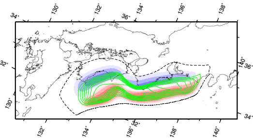
(c) Sub-slip 3 (Seismogenic + Down-dip)
