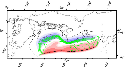
(b) Sub-slip 2 (Up-dip + Seismogenic)
