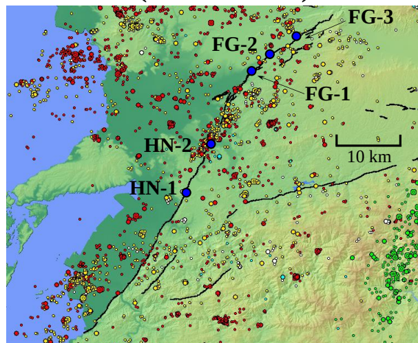
Futagawa and Hinagu faults (FG and HN)
