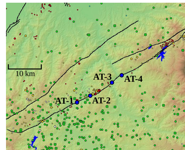
Atotsugawa Fault (AT)
