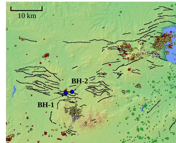
Beppu-Haneyama Fault (BH)
