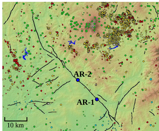
Atera Fault (AR)
