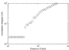
M: Red River Fault Zone
