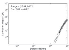
D: Andaman Basin
