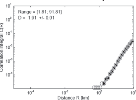
C: Sagaing Fault Zone
