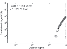
E: Sumatra Fault Zone
