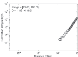
K: Song Da–Song Ma Fault Zones
