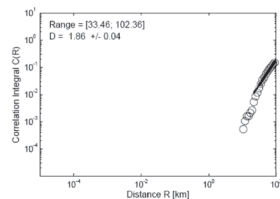
L: Xianshuihe Fault Zone
