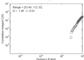
F: Hsenwi–Nanting Fault Zone
