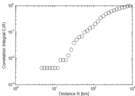
I: Jinghong–Mengxing Fault Zones
