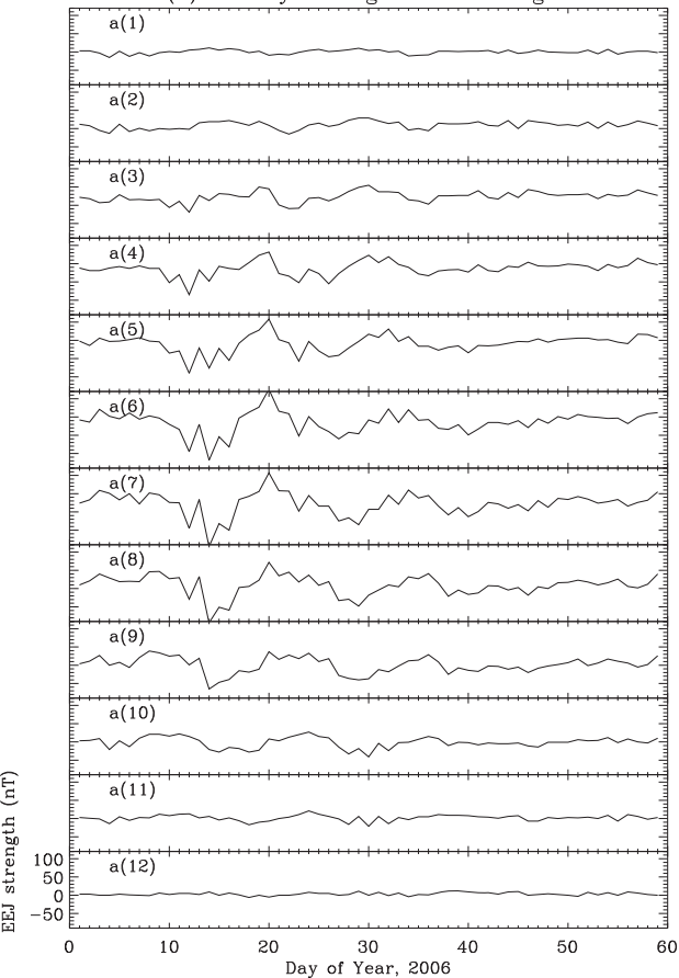
(a): Hourly averaged EEJ-strength
