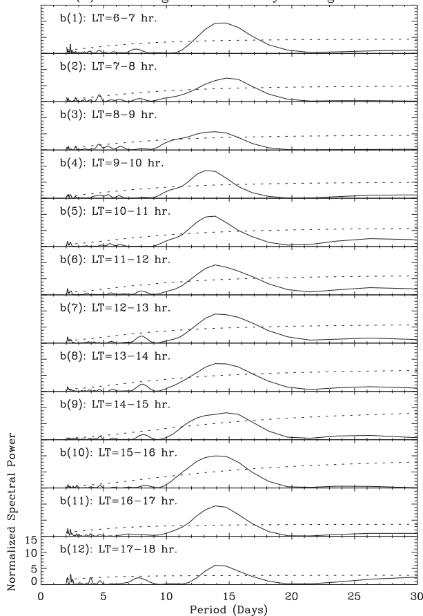
(b): Periodograms of hourly averaged EEJ
