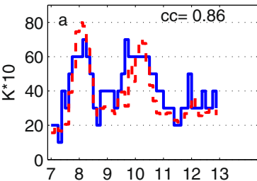
08–12 Nov. 2004 Storm
