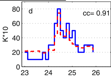
24–26 August 2005 Storm
