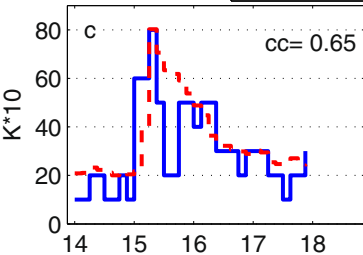
15–18 May 2005 Storm
