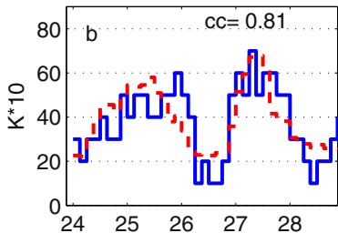
24–28 July 2004 Storm
