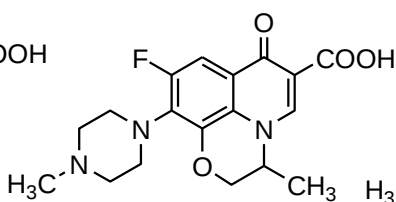
3 , Ofloxacin
