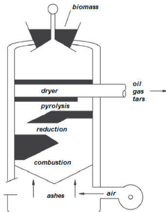
DOWNDRAFT
