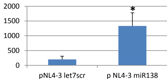
miR138
