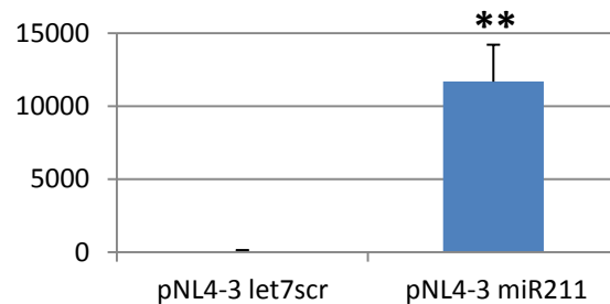
miR211
