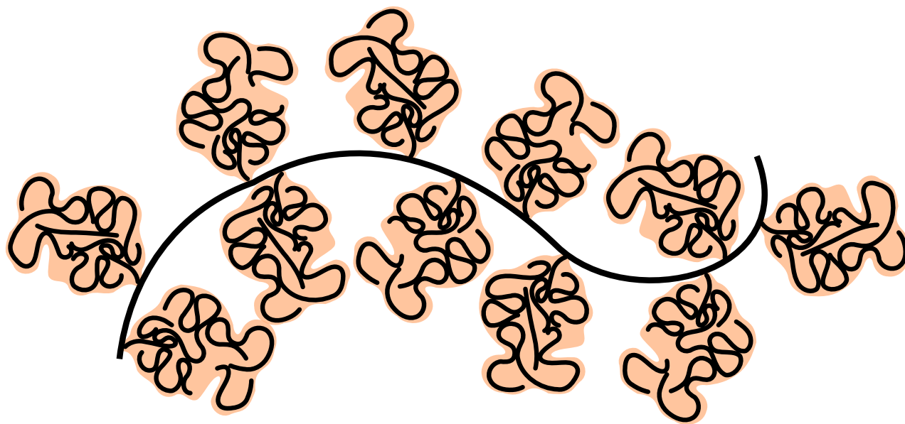
(c) Random Walk / Giant Loop \sim 1\text{-}3\text{ Mbp}
