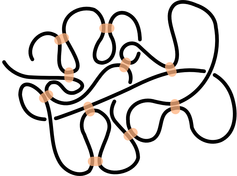
(a) Random Loop > 150\text{kbp}
