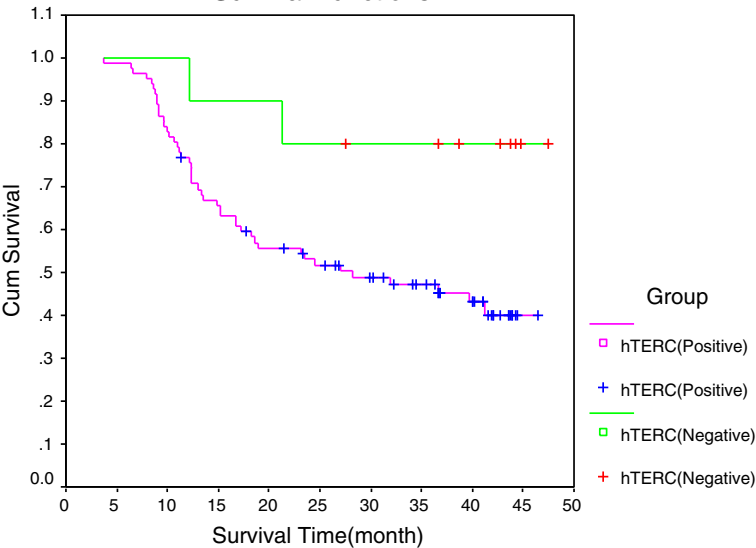
Survival Functions
