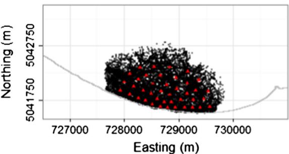
b) Positions retained ( HPE \leq 8 )
