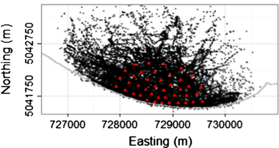
a) All positions
