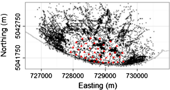
c) Positions removed ( HPE > 8 )
