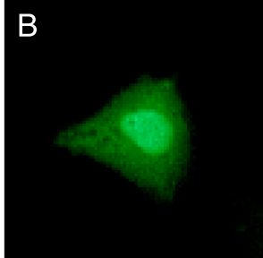
PHF1b \Delta 1
