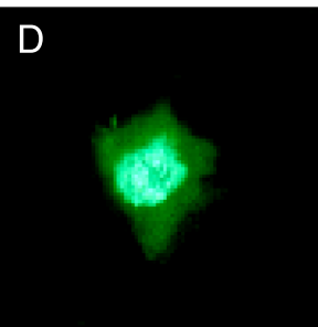
PHF1b \Delta 6
