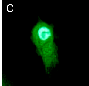
PHF1b \Delta 5
