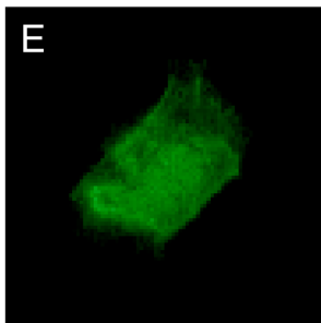
PHF1b \Delta 3
