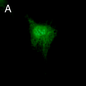
PHF1b
