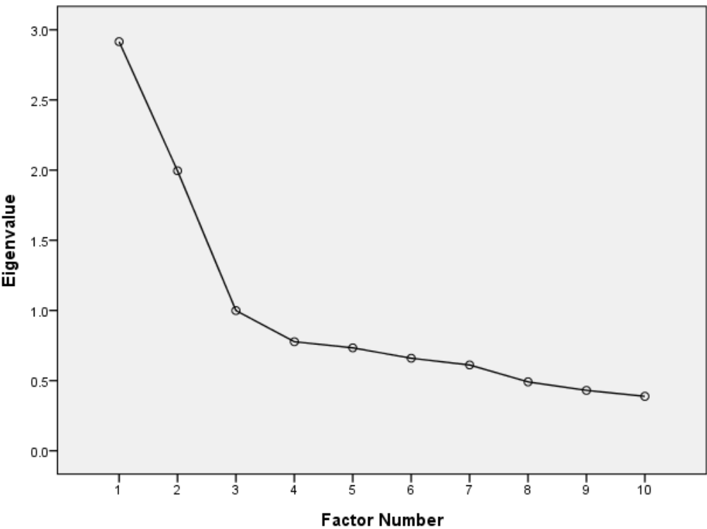
Scree Plot
