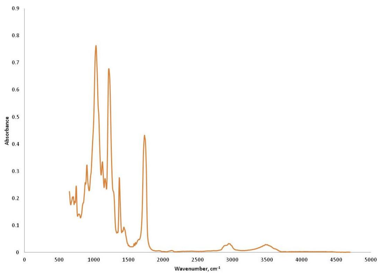
ATR-FTIR spectrum of cellulose acetate
