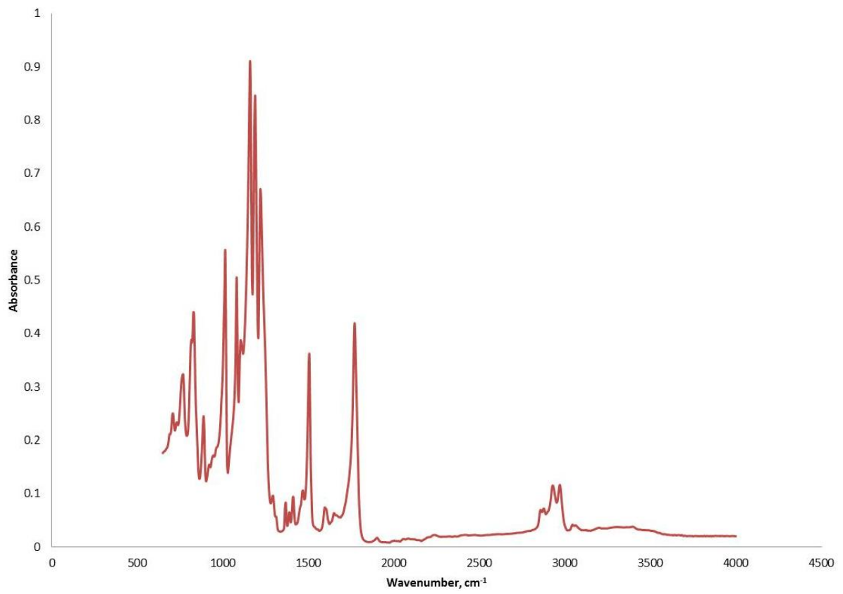
ATR-FTIR spectrum of polycarbonate
