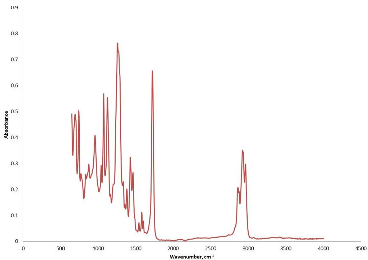
ATR-FTIR spectrum of poly (vinyl chloride)
