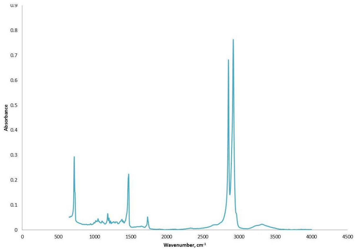
ATR-FTIR spectrum of polyethylene
