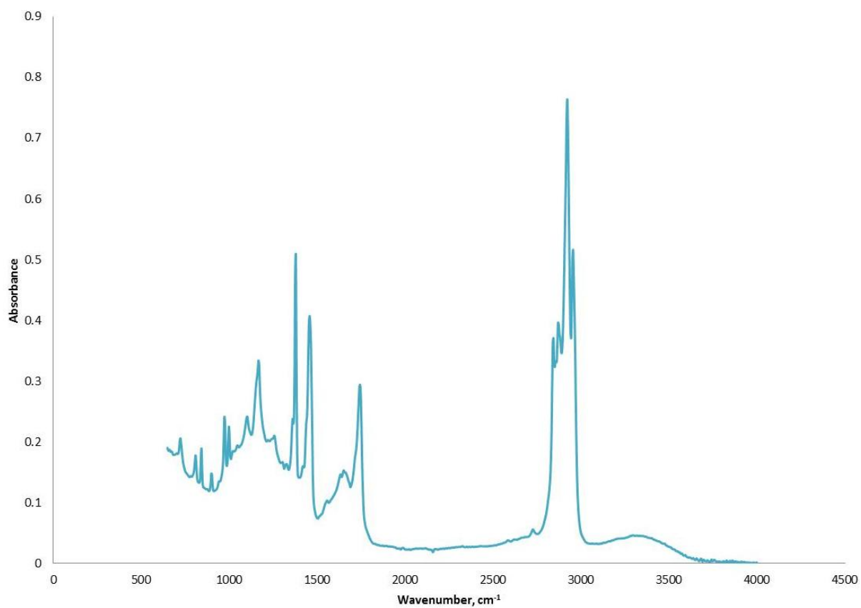
ATR-FTIR spectrum of polypropylene
