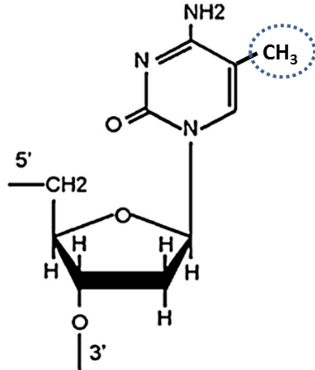
5-Methyl-Cytidine
