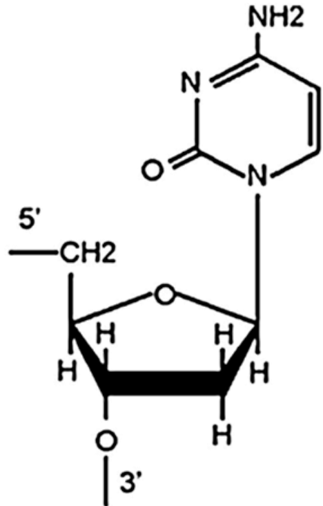
Deoxycytidine
