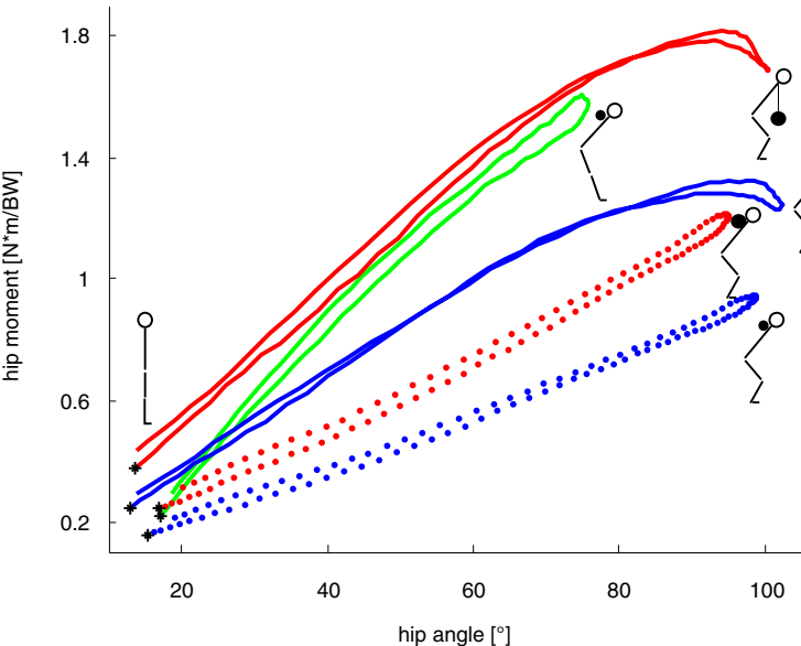
Hip moment as a function of the hip angle
